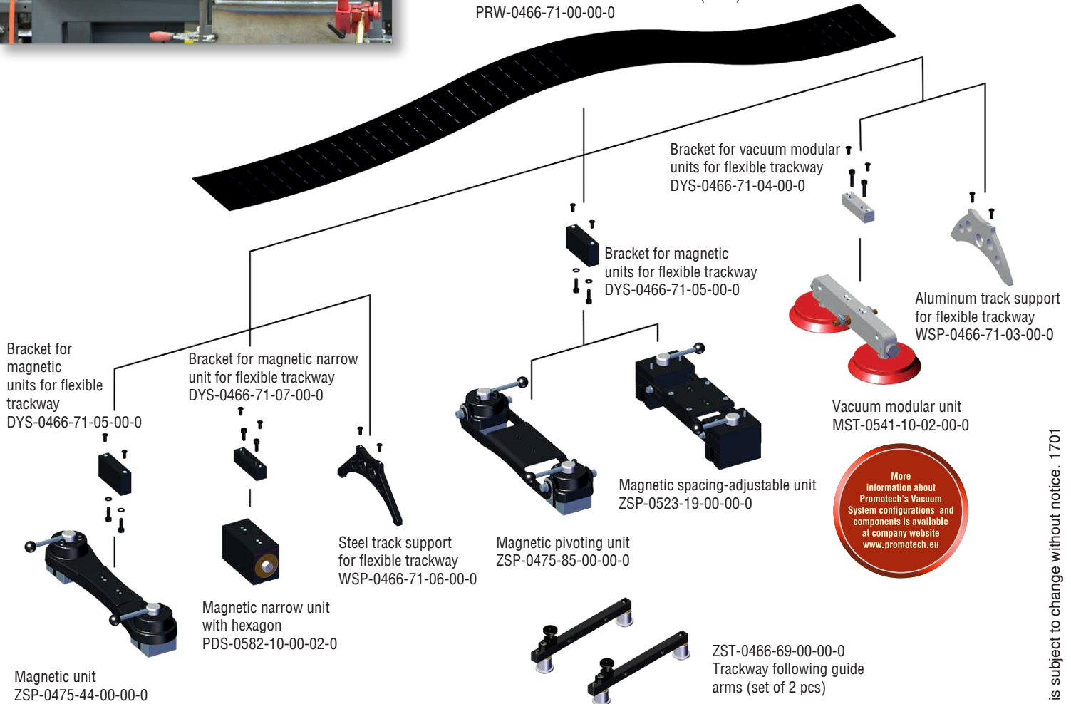
Flexible trackway length 1.88 m (6.1 ft). Minimum curvature radius of 1.25 m (4.1 ft) PRW-0466-71-00-00-0
